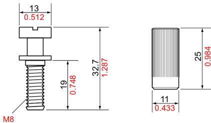
TonePros T1Z - Metric Tailpiece (Locking Stop Bar)
