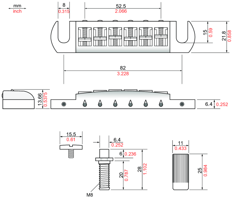
TonePros AVT2M - Wraparound Bridge with MSPRS Locking Studs (Metric)
