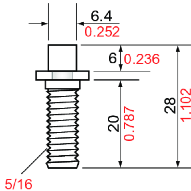
TonePros AVT2P- Wraparound Bridge with SPRS2 Locking Studs (USA P-Style)
