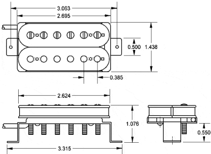
Seymour Duncan Whole Lotta Humbucker Pickups (SH-18) - without Cover
