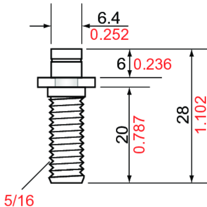
TonePros SS1 - Standard Brass Locking Studs
