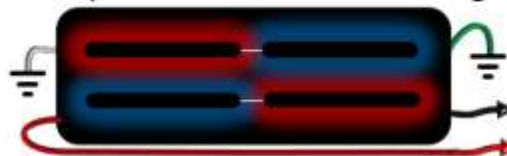
2J Squared Parallel Hum Canceling
