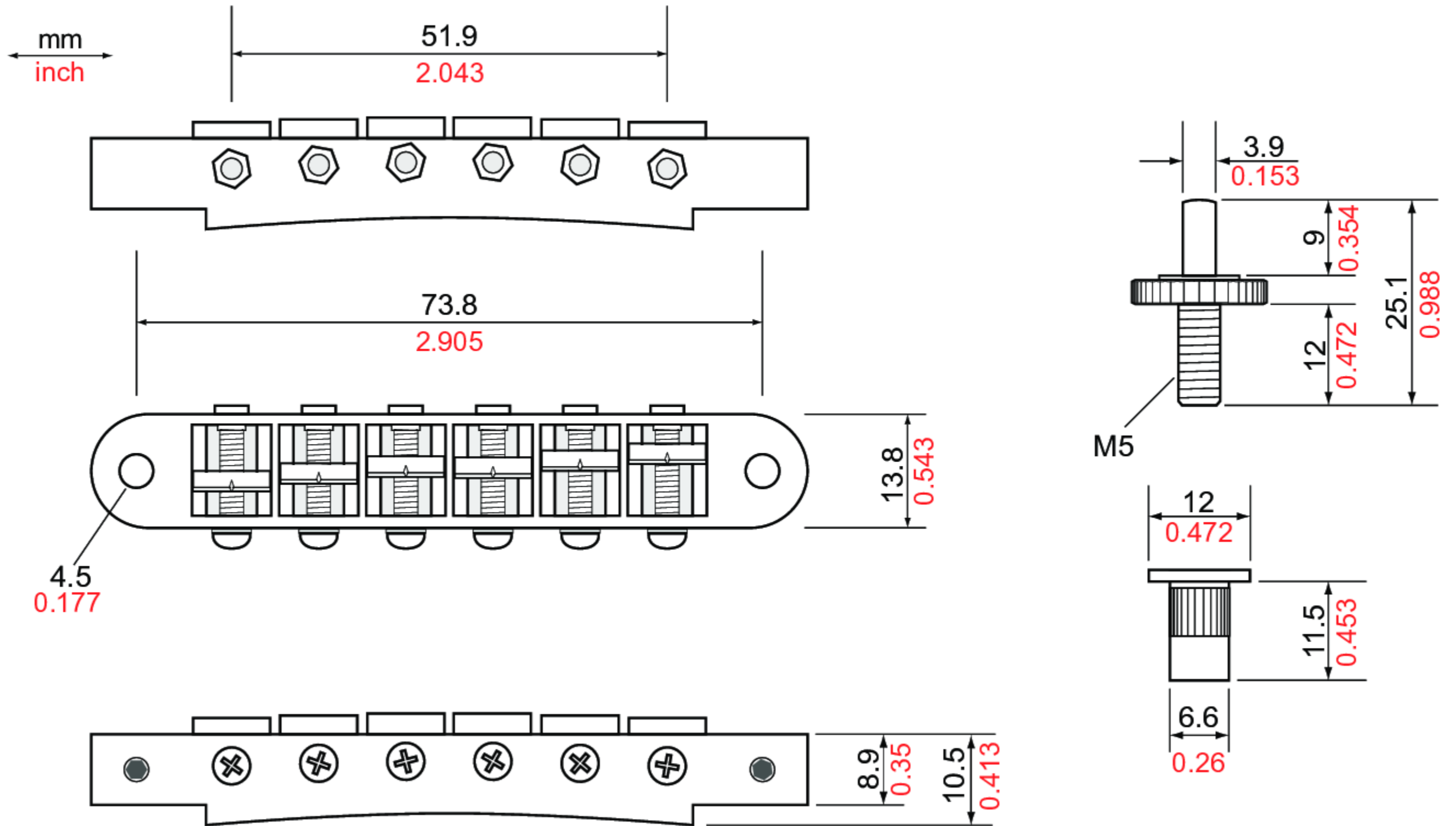
TonePros T3BP - Standard Tune-O-Matic Bridge (Small Posts / Notched Saddles)
